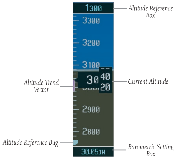
Figure 3.4.6 Altimeter
