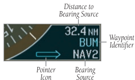
Figure 3.4.22 BRG2 Information Window
