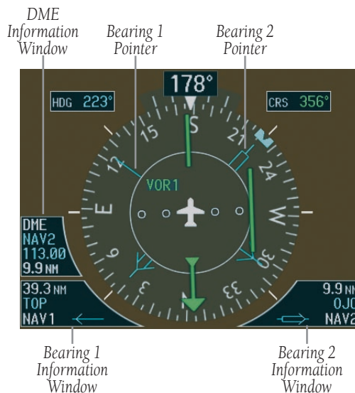
Figure 3.4.20 HSI with Bearing Information
