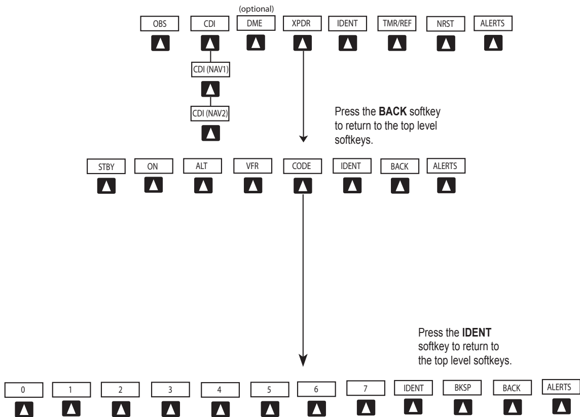
Figure 3.3.5 PFD Softkey Flow Chart – 3
