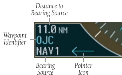
Figure 3.4.21 BRG1 Information Window
