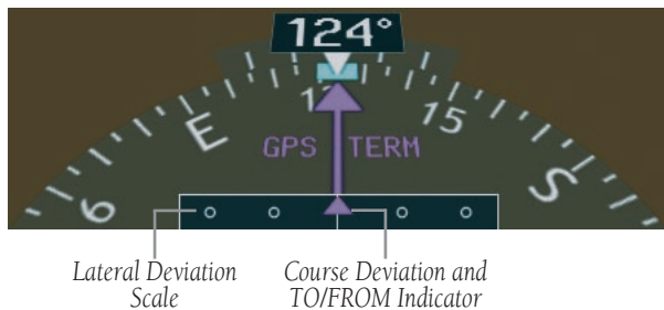
Figure 3.4.14 ARC HSI
